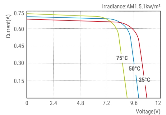
SLP005-06U I-V Curves
